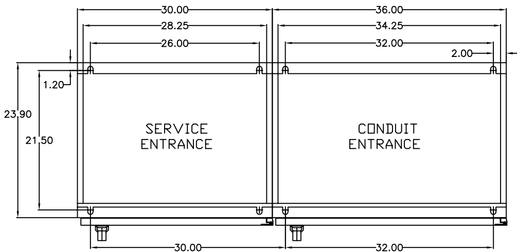
BASE PLAN
