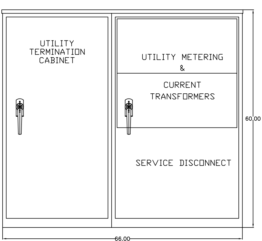
PANEL ELEVATION
