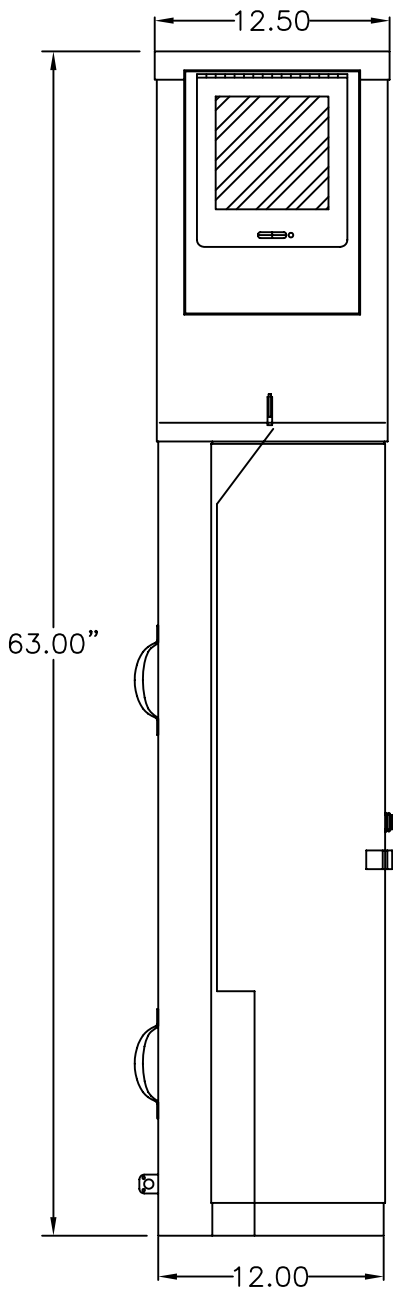
FRONT VIEW
