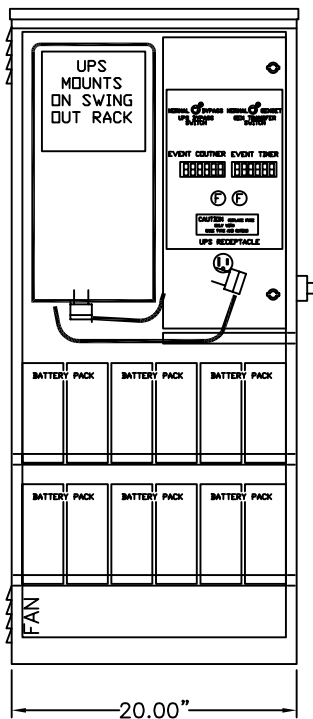
BACK VIEW
