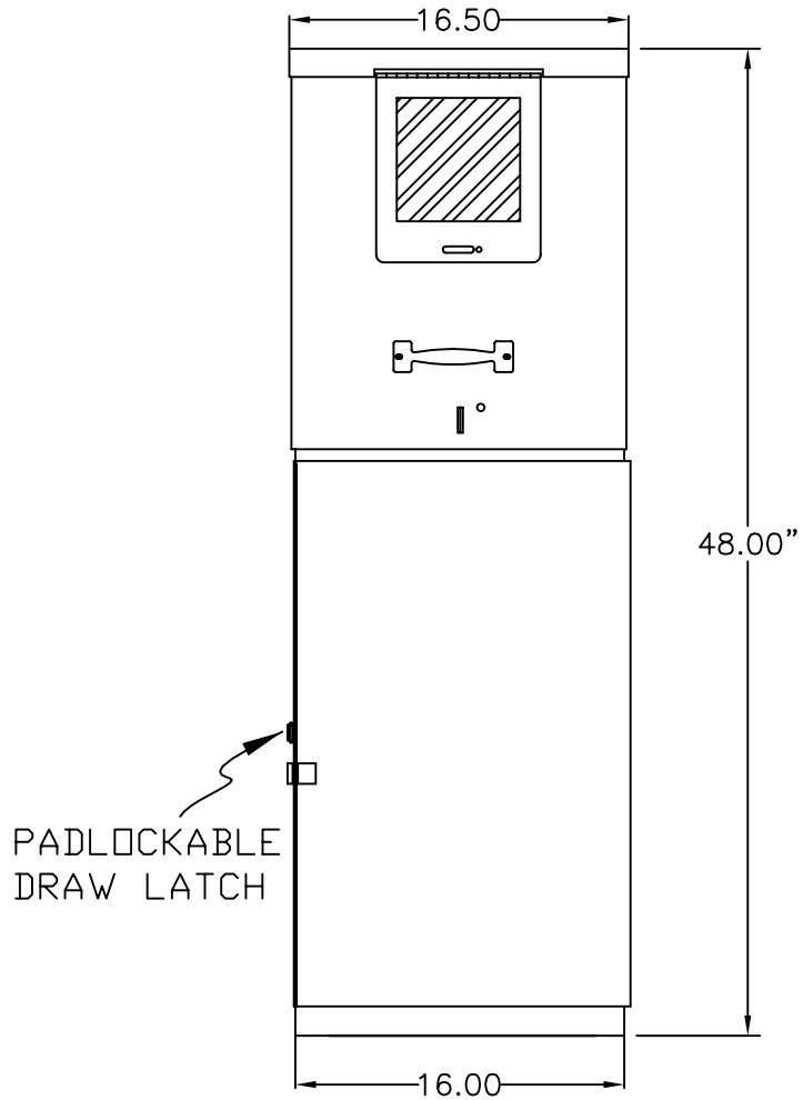
FRONT VIEW
